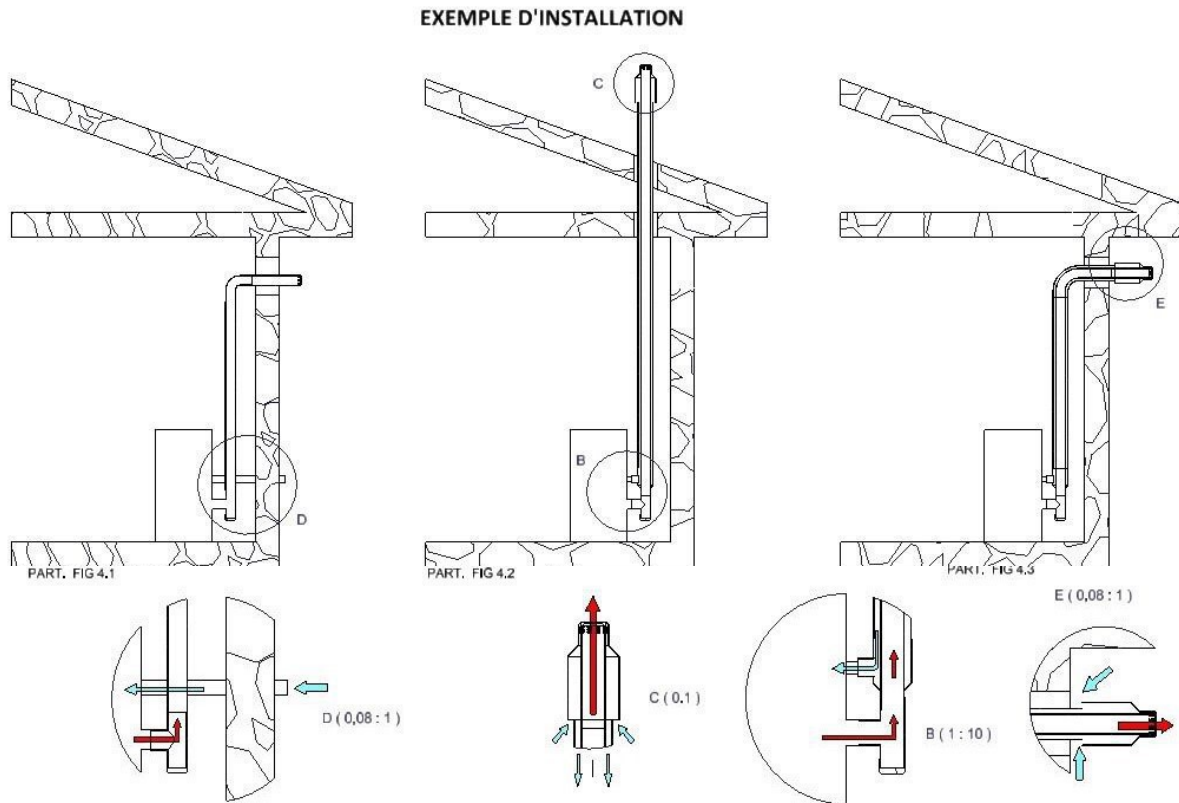
Figure 4 – Configurations d'installation possibles
